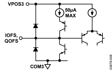
Figure 8. Circuit F
